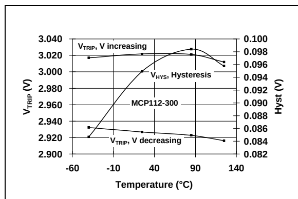
FIGURE 2-8: V_{TRIP} and V_{HYST} vs. Temperature ( MCP112-300 ).
