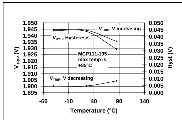
FIGURE 2-7: V_{TRIP} and V_{HYST} vs. Temperature ( MCP111-195 ).
