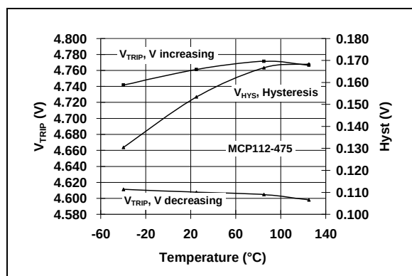
FIGURE 2-9: V_{TRIP} and V_{HYST} vs. Temperature ( MCP112-475 ).
