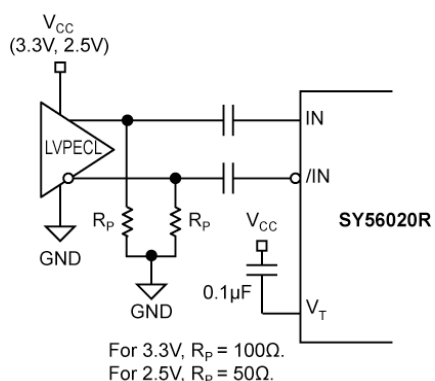
Figure 4d. LVPECL Interface (AC-Coupled) For 3.3V, R_P = 100\Omega . For 2.5V, R_P = 50\Omega .
