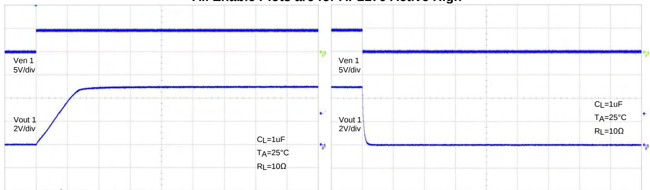
Channel 1 Turn-On Delay and Rise Time
