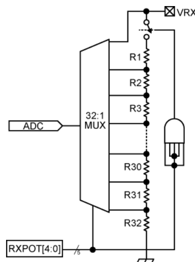
Figure 4. RXPOT Block Diagram
