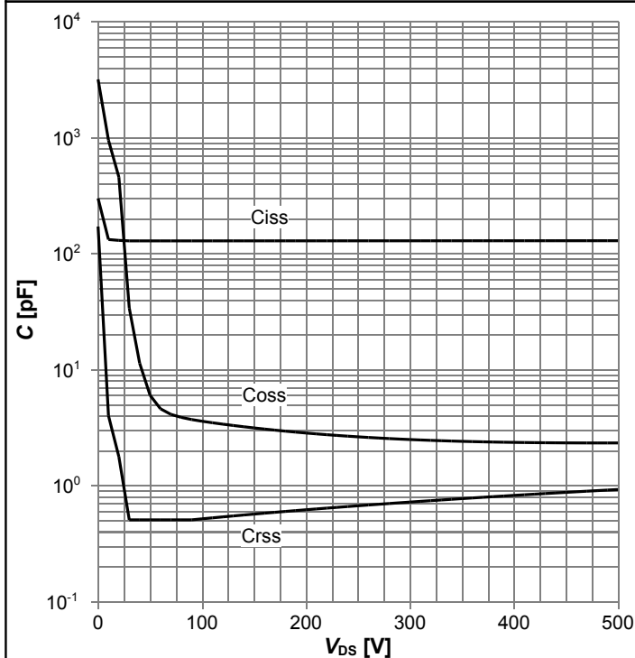
Diagram 14: Typ. capacitances
