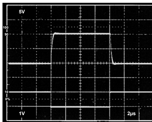
Figure 40. Combination Amplifier Transient Response
