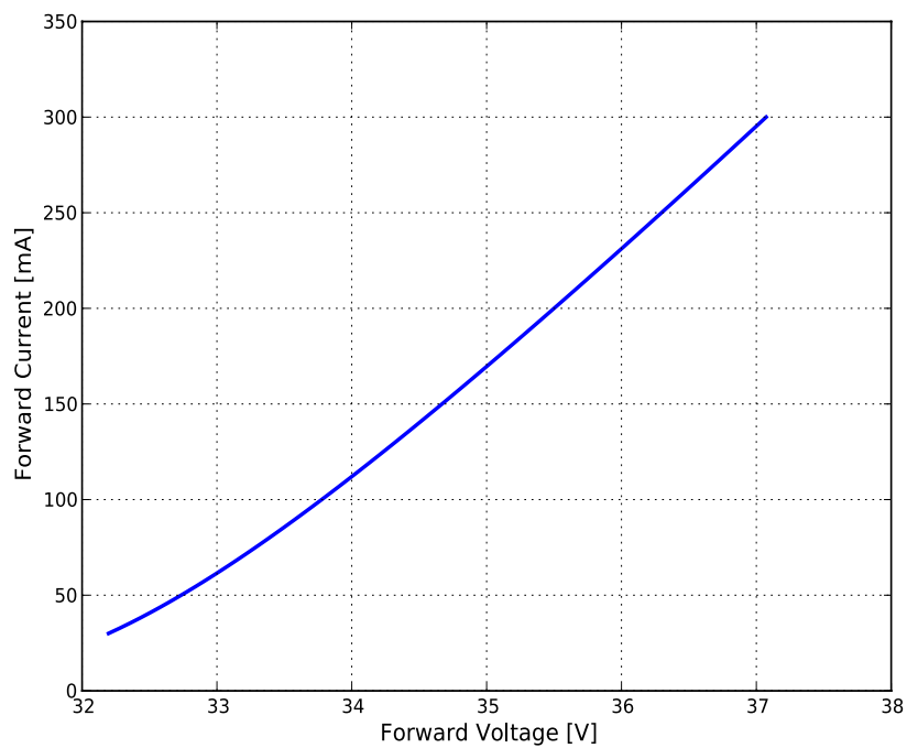
Figure 4b. Typical forward current vs. forward voltage for L2C3-xxxx207E06000 at T_j=85^{\circ}\text{C} .
