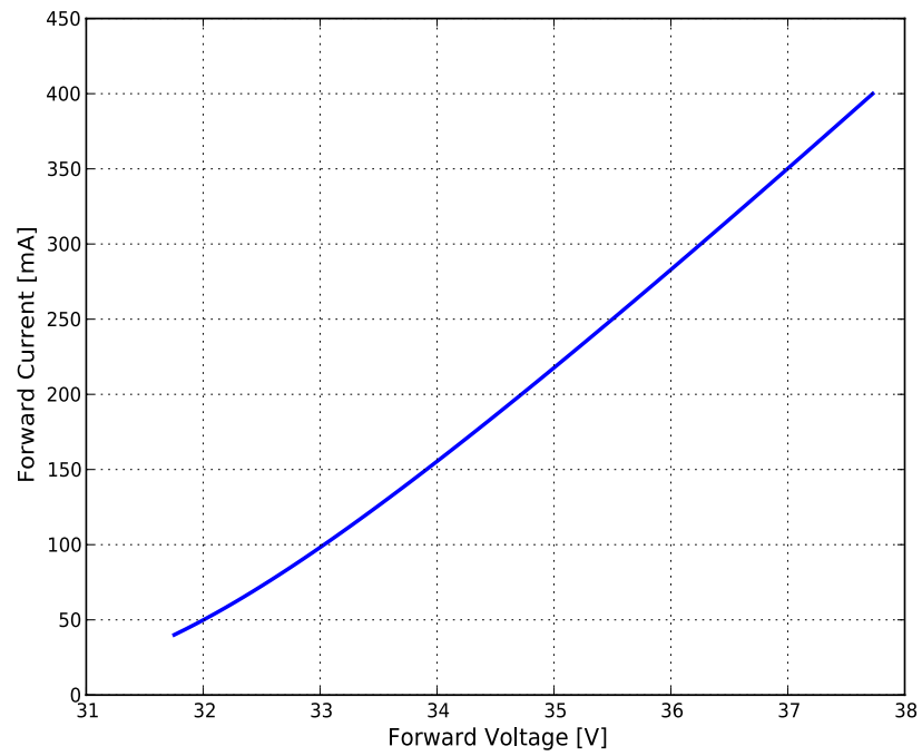
Figure 4c. Typical forward current vs. forward voltage for L2C3-xxxx209E06000 at T_j = 85^\circ\text{C} .
