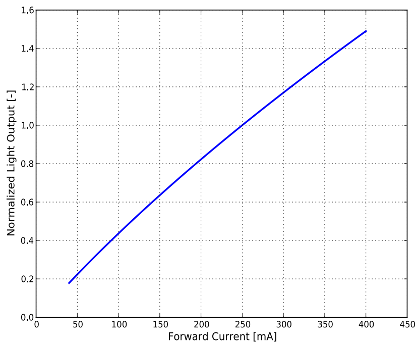
Figure 3c. Typical normalized light output vs. forward current for L2C3-xxxx209E06000 at T_j=85^{\circ}\text{C} .
