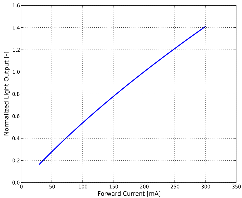
Figure 3b. Typical normalized light output vs. forward current for L2C3-xxxx207E06000 at T_j=85^{\circ}\text{C} .
