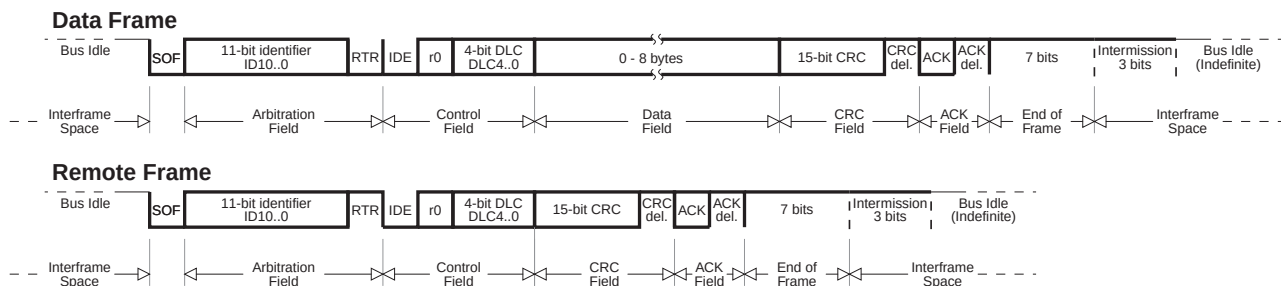
Figure 43. CAN Standard Frames
