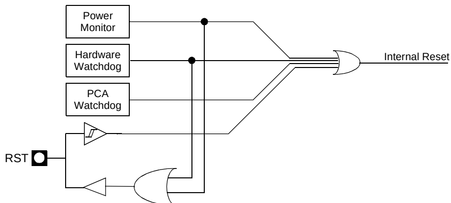
Figure 16. Reset Schematic
