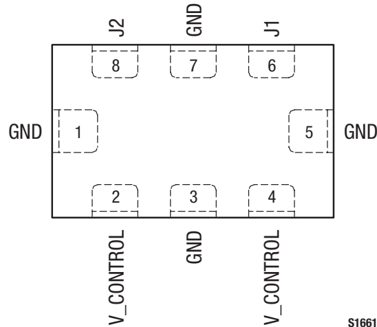
Figure 2. SKY12236-11 Pinout – 8-Pin MCM (Top View)
