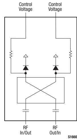
Figure 1. SKY12236-11 Block Diagram
