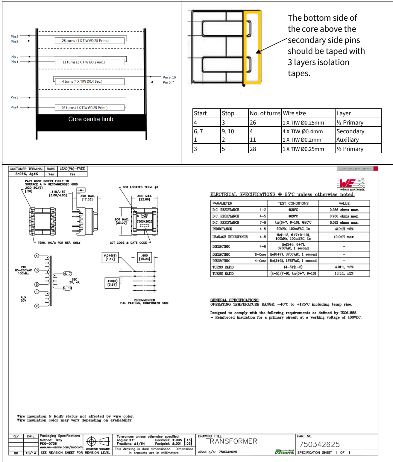
Figure 5 Transformer structure
