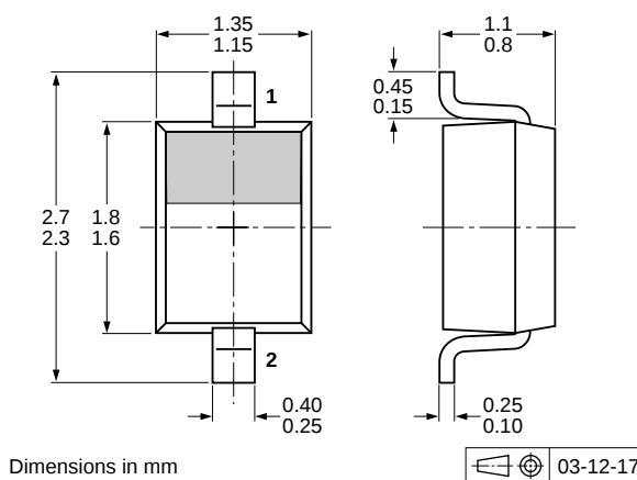
Fig 8. Package outline SOD323 (SC-76)
