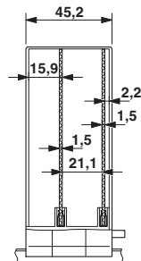
Internal housing dimensions, electronics housing ME 45 BUS...
