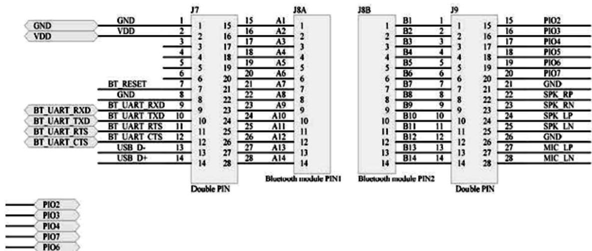
Figure 12: Audio input and output Schematic diagram
