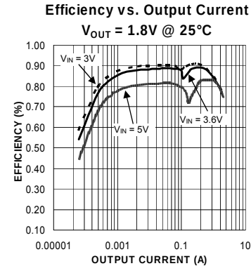
Figure 2. Efficiency Under Load
