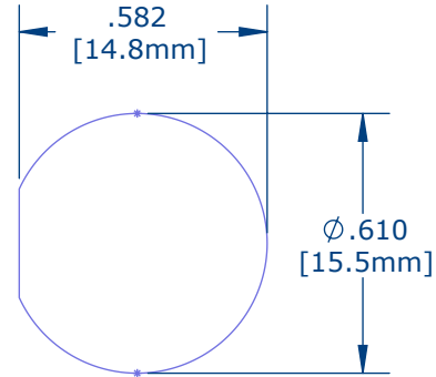
RECOMMENDED PANEL CUT-OUT TOLERANCE: ±.003
