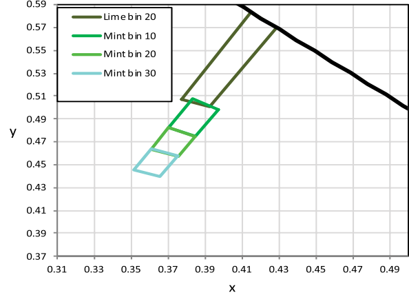
Figure 8. Color Bin Structure for LUXEON 2835 Lime and Mint for Table 7.
