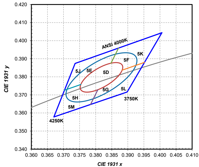
Figure 10b. 1/9 th color bin structure for LUXEON 2835E and LUXEON 2835C 4000K at test current and binning temperature of T_j=25^{\circ}\text{C} .
