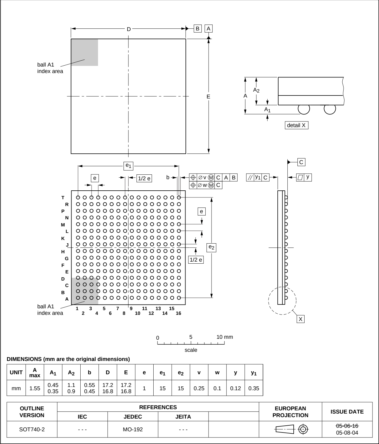
Fig 45. Package outline of the LPGA256 package
