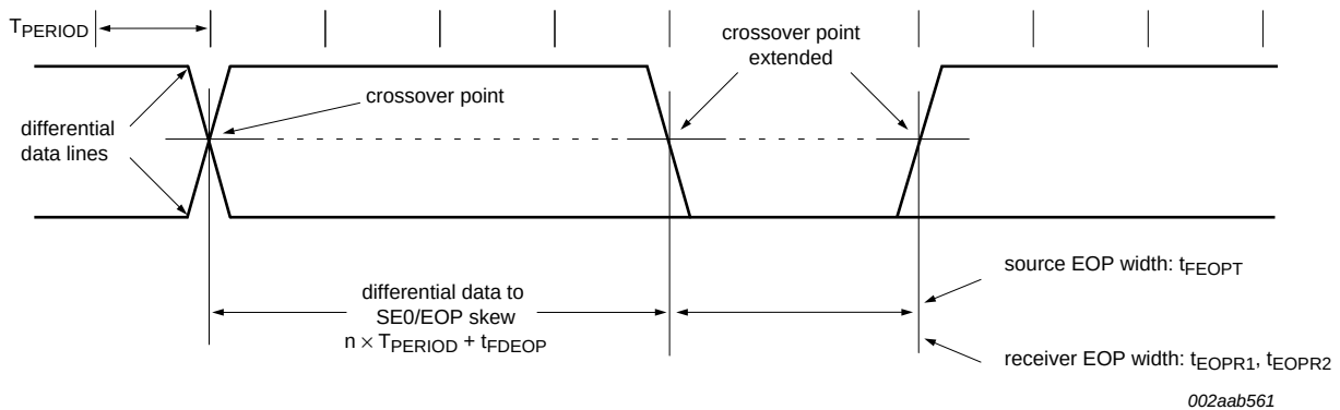
Fig 34. Differential data-to-EOP transition skew and EOP width
