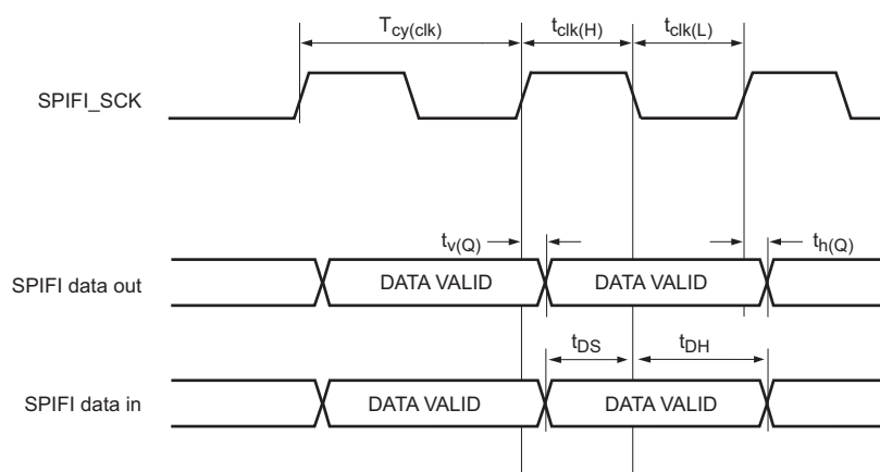
Fig 37. SPIFI timing
