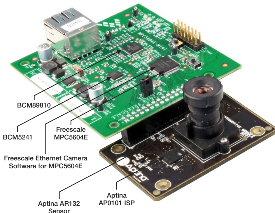
Figure 1: Qorivva MPC5604EKIT
