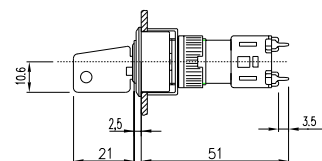
46 keylock switch 2 positions for flush mounting 51 - 79 mm, keylock switch with 3 positions for flush mounting 51 - 54 mm page 612, 616
