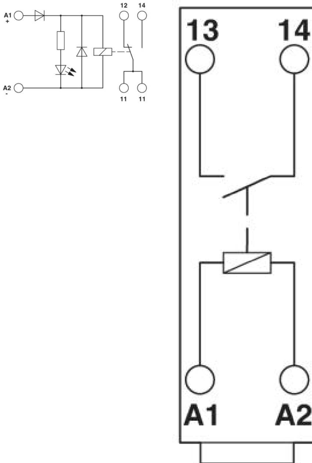
Circuit diagram
