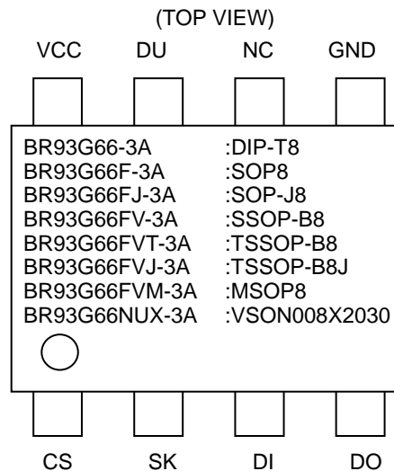
Figure 3. Pin Configuration
