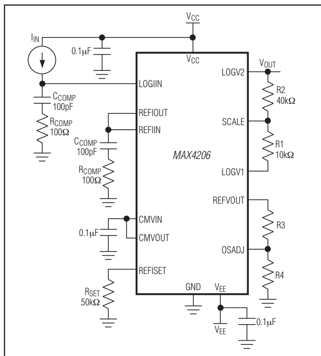
Figure 6. Dual-Supply Typical Operating Circuit
