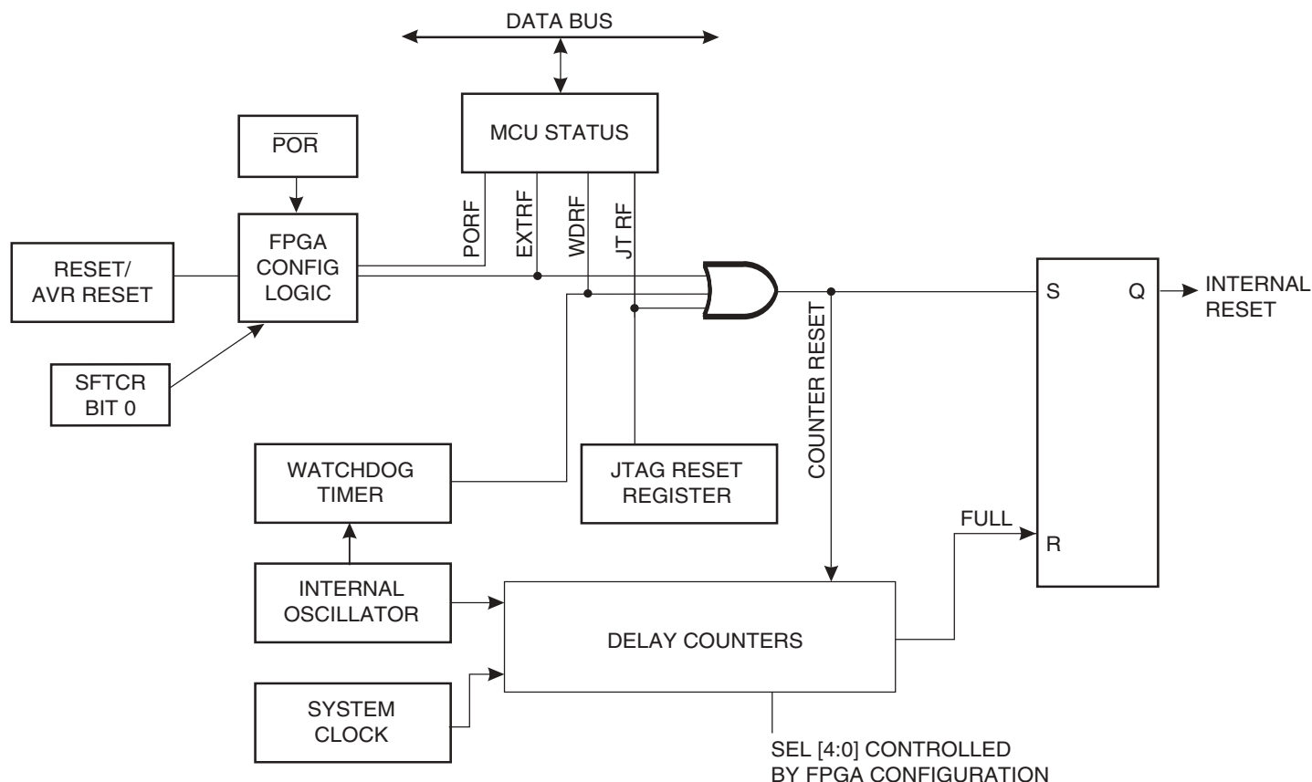
Figure 35. Reset Logic
