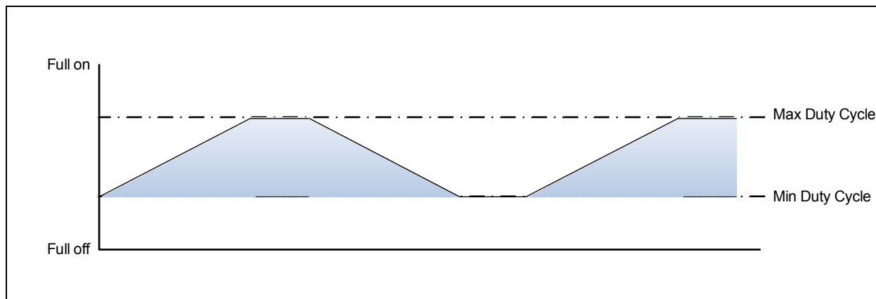
FIGURE 28-3: CLIPPING EXAMPLE
