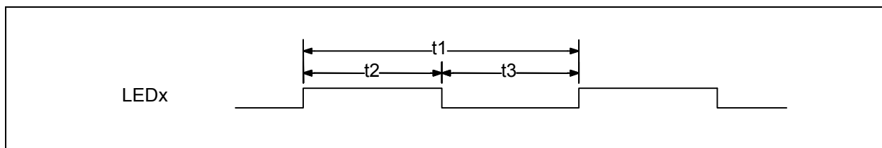
FIGURE 43-9: BLINKING/BREATHING PWM OUTPUT TIMING
