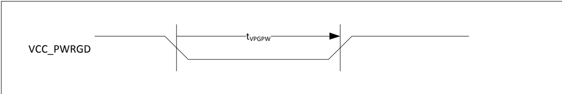
FIGURE 43-1: VCC_PWRGD TIMING DIAGRAM
