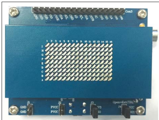
Figure 1: Photo of IS31FL3731 Evaluation Board (Note: Old version EVB please refer to Appendix 1)
