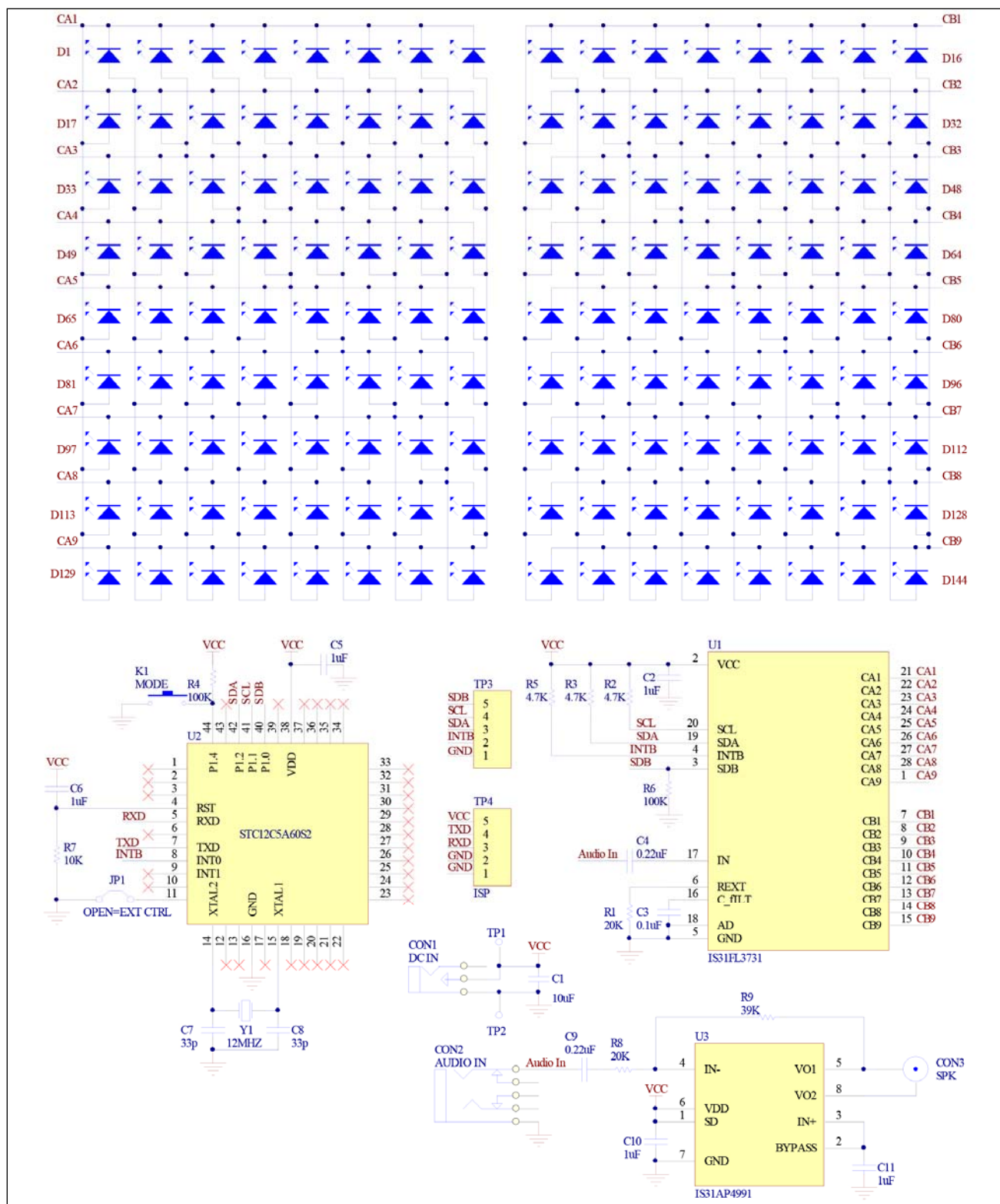
Figure 13: IS31FL3731 Application Schematic
