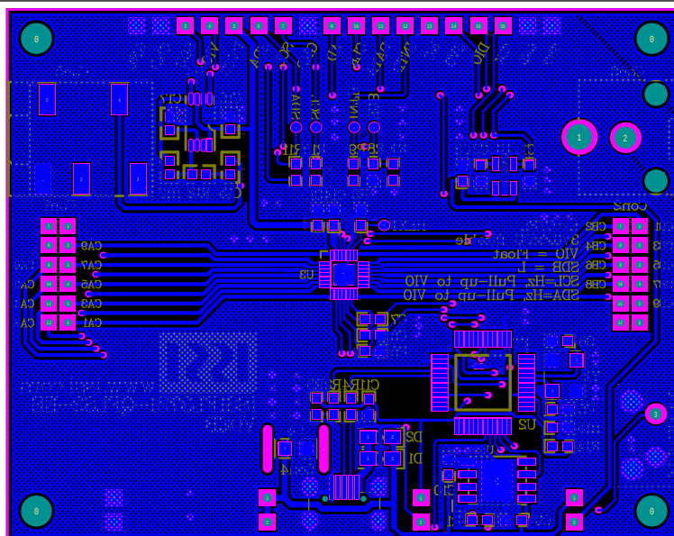
Figure 7: Board PCB Layout - Bottom Layer
