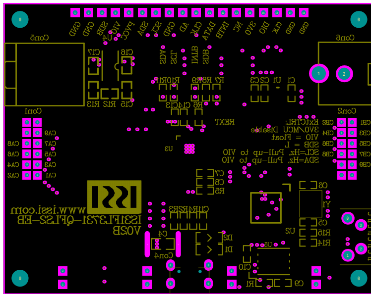
Figure 6: Board Component Placement Guide - Bottom Layer
