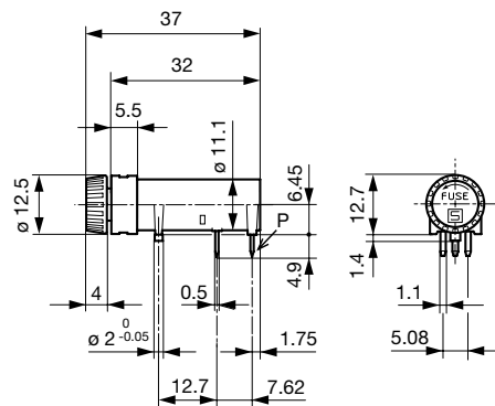
Variant Fingergrip 3101.0055 / Connector tinned
