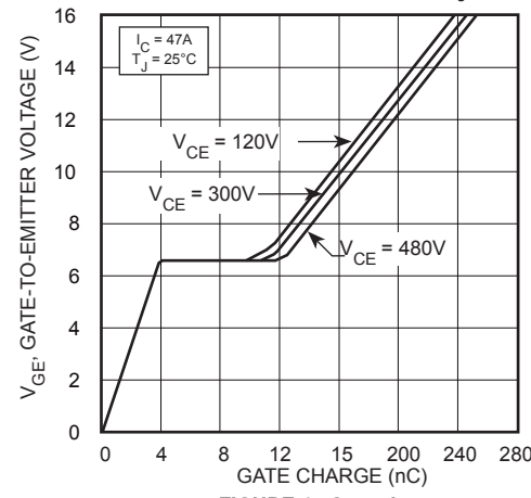
FIGURE 4, Gate charge
