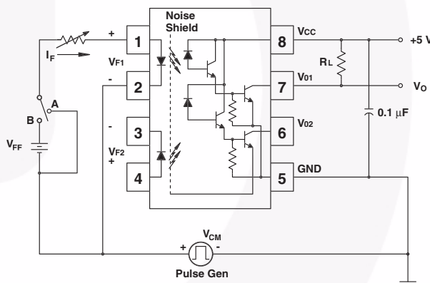
Test Circuit for HCPL-0730 and HCPL-0731
