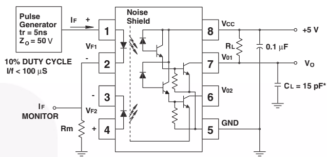
Test Circuit for HCPL-0730 and HCPL-0731
