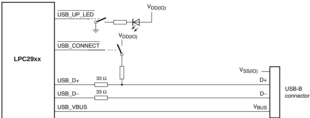
Fig 35. LPC2926/2927/2929 USB device port configuration
