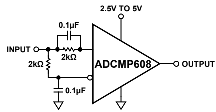
Figure 12. Self-Biased, 50% Slicer
