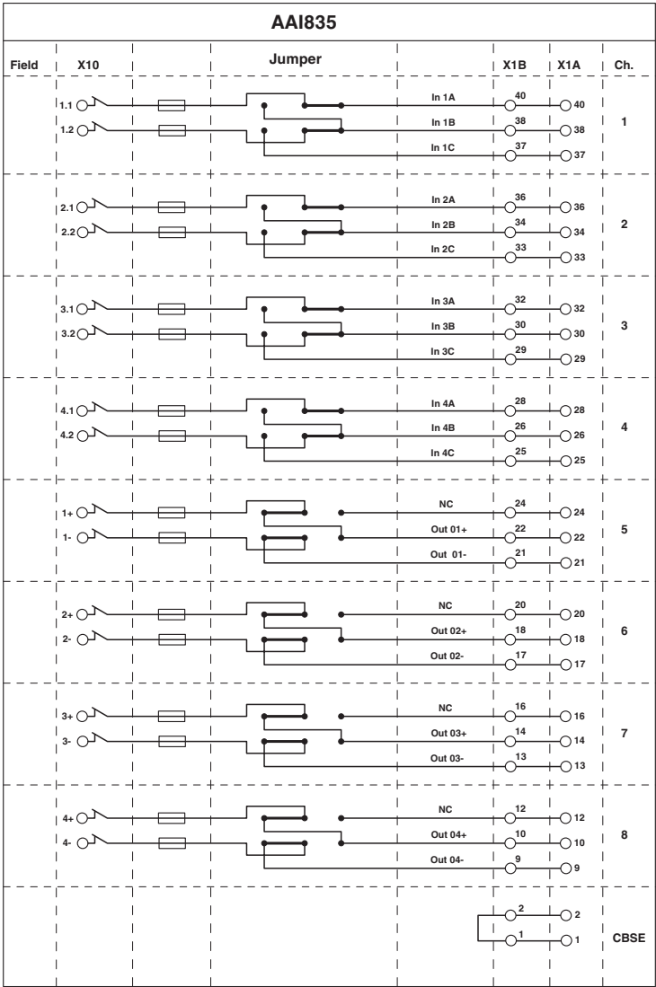
Circuit diagram
