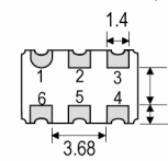
Underside View
