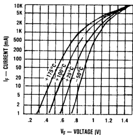
FIGURE 1 TYPICAL FORWARD VOLTAGE vs FORWARD CURRENT
