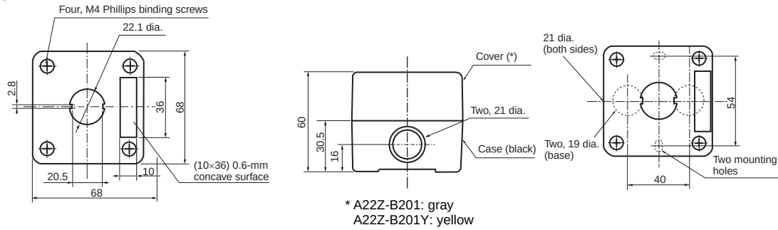
Cable Port Hole (Top View)
