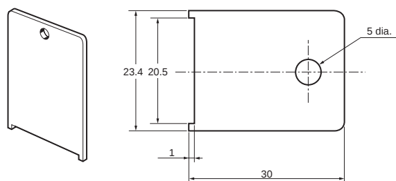
Cap Tightening Tool A22Z-3908
