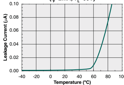
Typical Leakage Current vs. Temperature ( I_F=2mA, V_L=60V )
