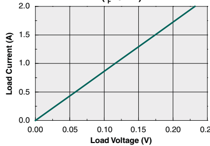
Load Current vs. Load Voltage DC-Only Configuration ( I_F=0mA )
