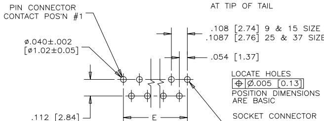
RECOMMENDED P.C.B. LAYOUT (COMPONENT SIDE OF BOARD)
