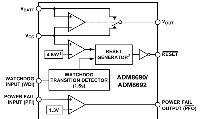
Figure 1. ADM8690/ADM8692
