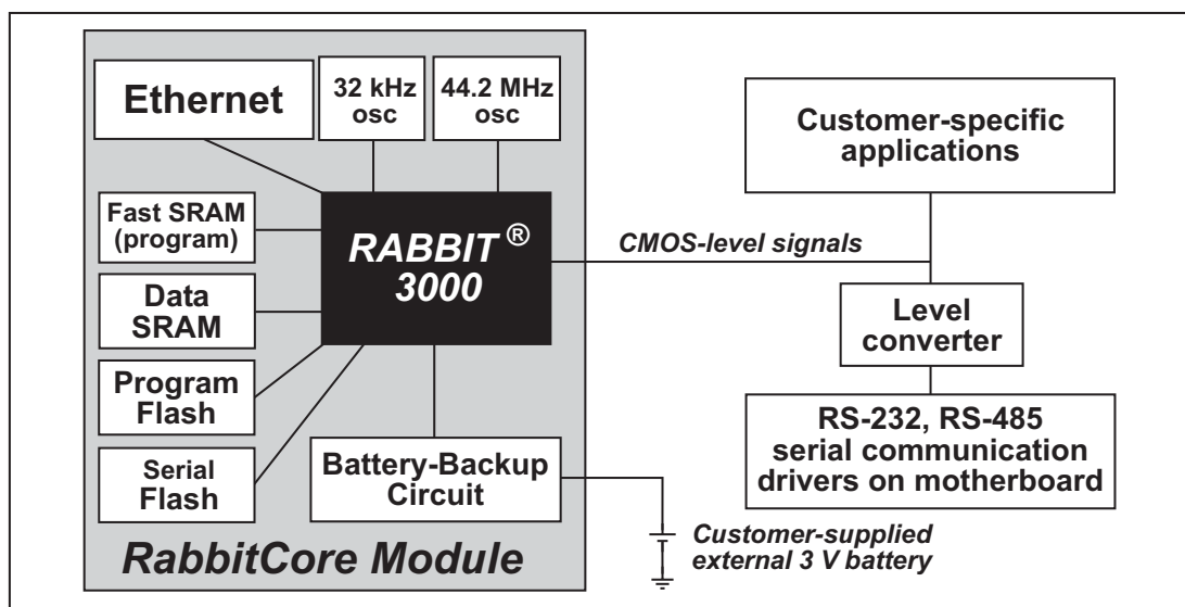
Figure 4. RCM3309/RCM3319 Subsystems
