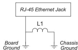
Figure 8. Ferrite Bead Isolation
