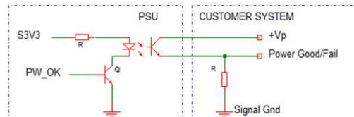
Figure 6: Isolated Signal Output connections
