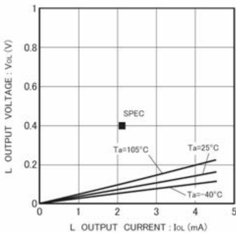
Figure 4. L output voltage V_{OL} - I_{OL} ( V_{CC}=4.0V )
