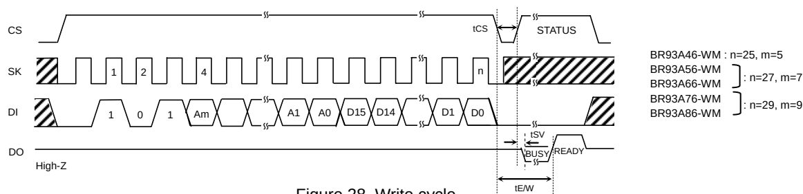
Figure 28. Write cycle
