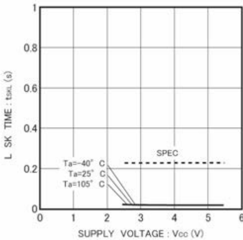
Figure 15. SK low time tSKL
