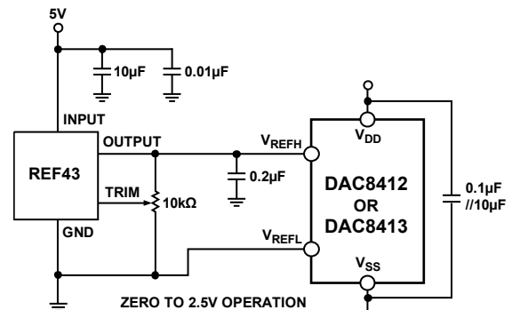
Figure 42. +5 V Single-Supply Operation
