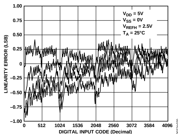
Figure 19. Channel-to-Channel Matching ( V_{SUPPLY} = +5\text{ V/GND} )
