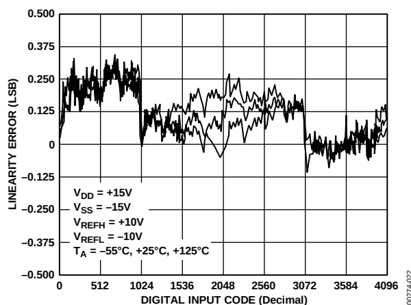
Figure 21. INL vs. Code
