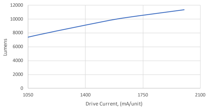
Lumens vs. Drive Current
