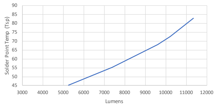
Tsp vs. Lumens
