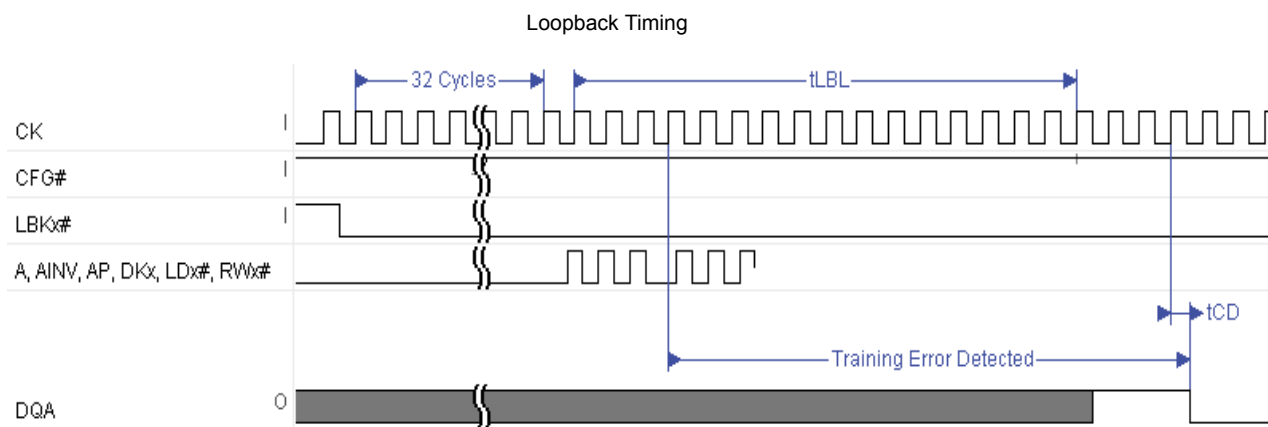
Figure 15. Loopback Timing
