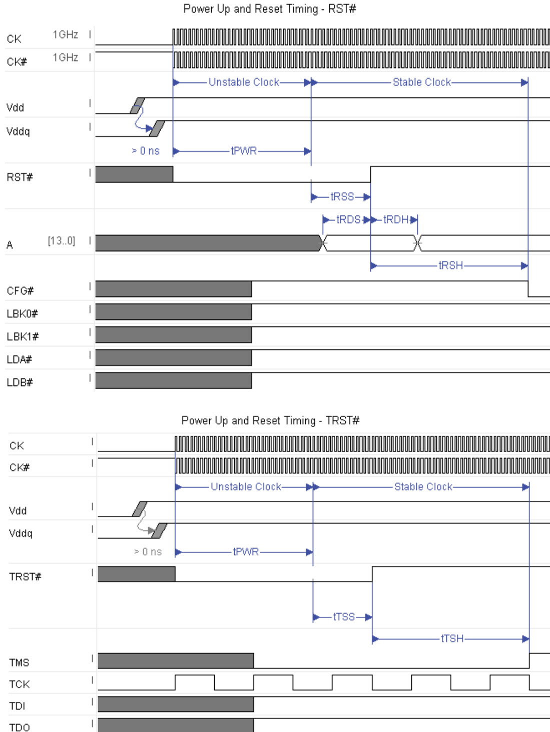
Figure 16. Reset Timings
