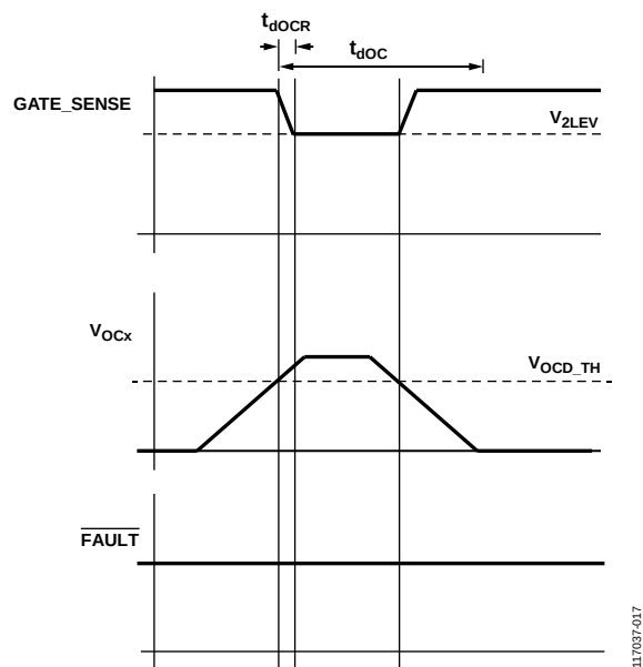
Figure 17. Two-Level Timer Recovery Example
