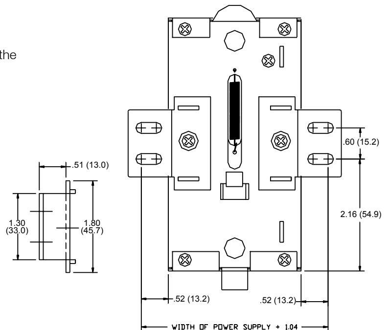
Dimensional Diagram - in (mm)
